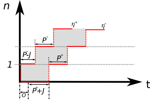
Figure 3.6.: \eta^+ and \eta^- Functions of Event Patterns
