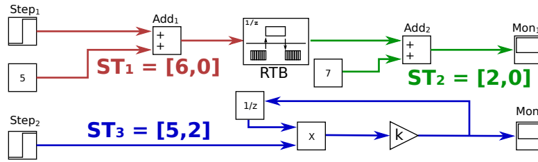
Figure 2.3.: Example for a Simulink Block Diagram
