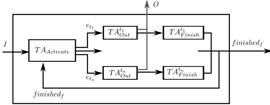
Figure 3.27.: Transition System Components
