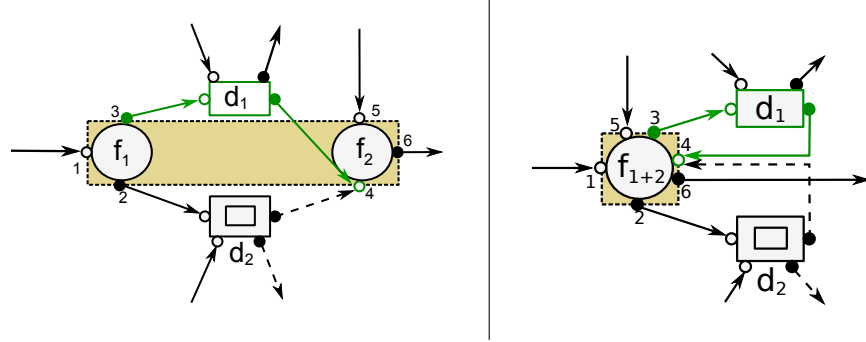
Figure 5.2.: Merging Function Nodes
