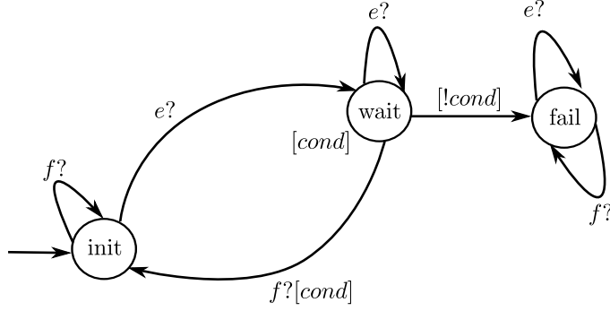
Figure 3.19.: Condition Pattern Automaton (RSL pattern 'F2' [65])
