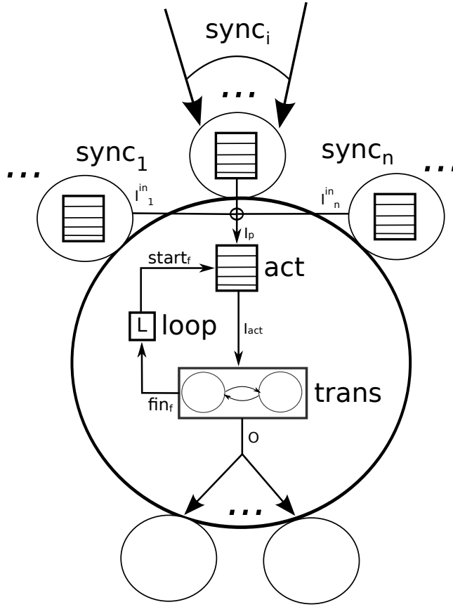
Figure 3.23.: Function Node Semantics - Overview
