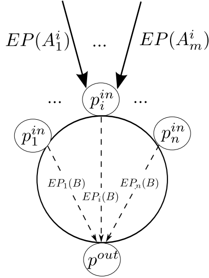
Figure 3.31.: Event Pattern Propagation using Causality Pattern
