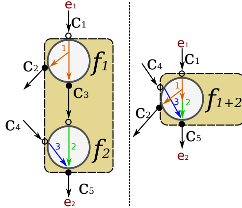
Figure 5.1.: Task Creation Example for a Task Chain
