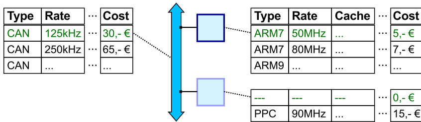
Figure 6.2.: Examples for Modification Rules (Source:[11])
