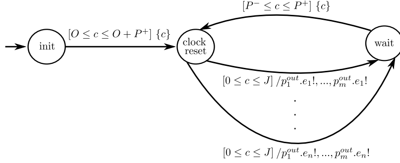
Figure 3.20.: Complex Transitions for Timed Automata
