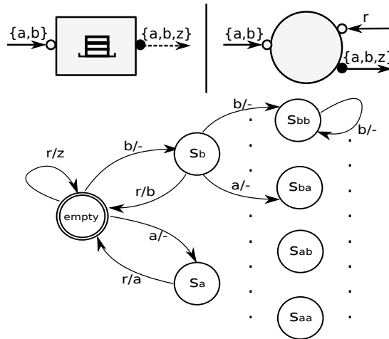
Figure 3.10.: Translation of FIFO Data Node
