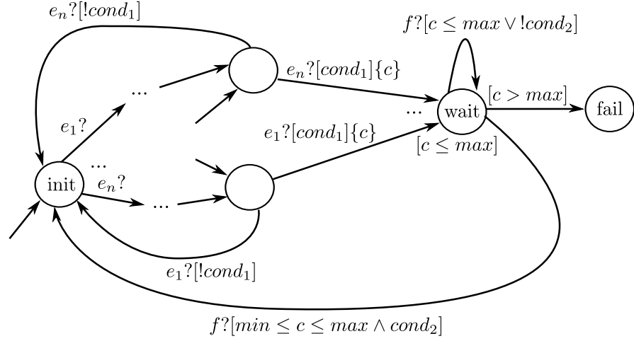
Figure 3.18.: Causality Pattern Automaton
