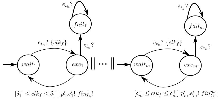
Figure 3.29.: Output Automata Composition TA_{Out}^{t_k} for Transition t_k
