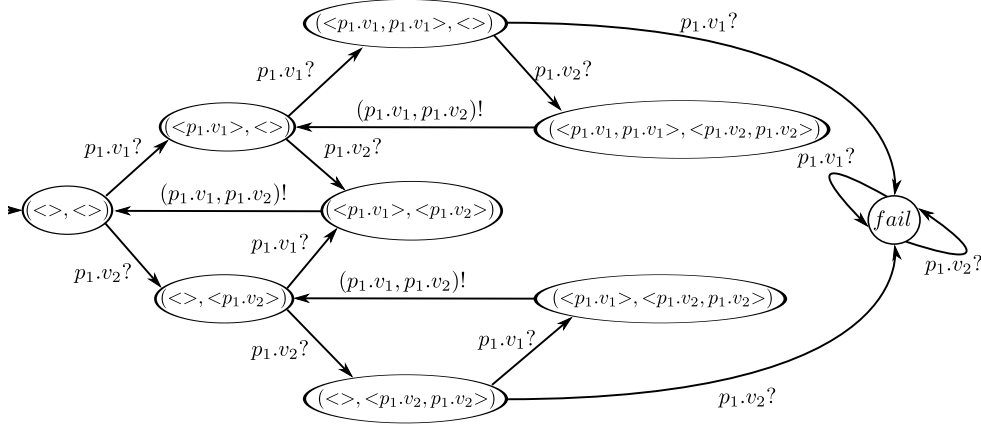
Figure 3.25.: Synchronization Buffer Automaton with capacity c = 2
