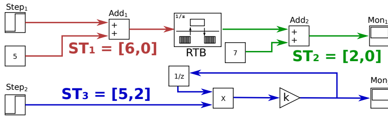
(a) Simple Example of a Simulink Block Diagram
