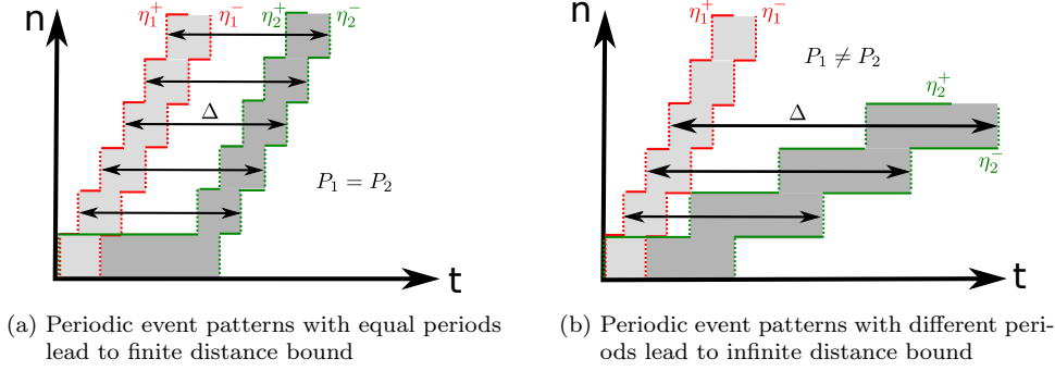
Figure 3.32.: Deciding boundedness for periodic event patterns
