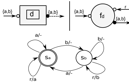
Figure 3.9.: Translation of Shared Data Node
