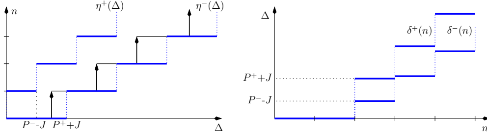
Figure 2.1.: Periodic/Sporadic event stream model (Source: [24])
