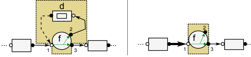
Figure 5.3.: Elimination of Local Data Nodes
