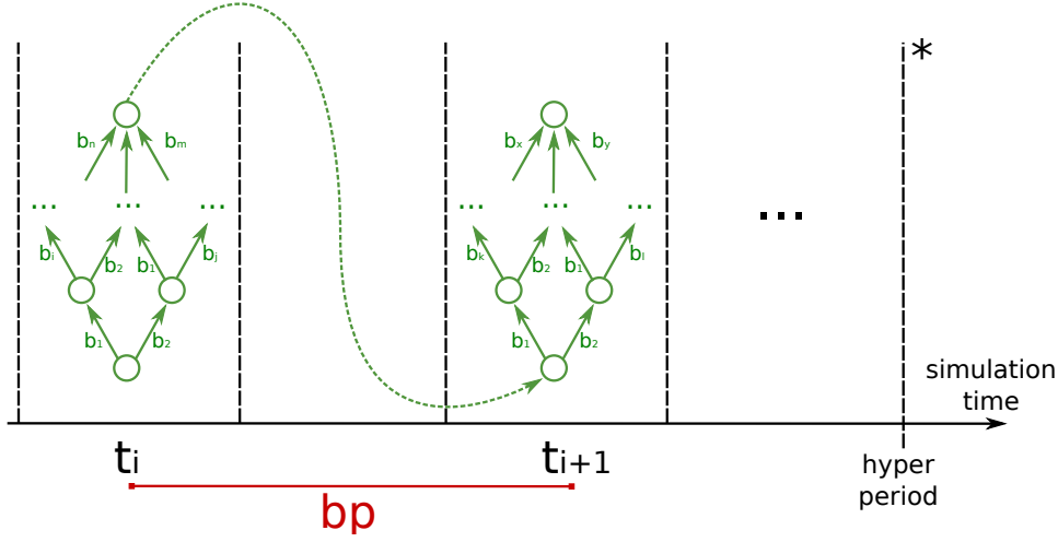
Figure 4.2.: Simulink Execution Semantics
