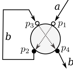
Figure 3.14.: Example of a Superposition (OR) Loop
