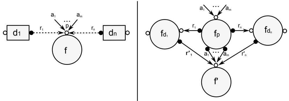
Figure 3.8.: Left: Read channels from Data Nodes d_1 to d_n Right: Translation of Read Channels into Basic Function Network
