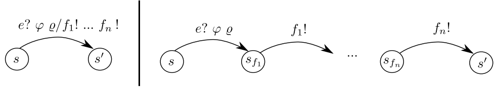
Figure 3.20.: Complex Transitions for Timed Automata
