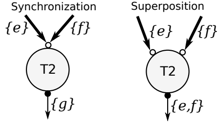
Figure 3.1.: Task Activation by Synchronization (AND) and Superposition (OR)
