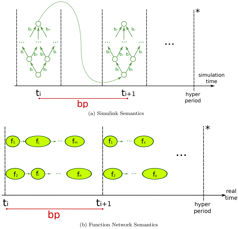
Figure 4.4.: Preserving Semantics from Simulink to Function Networks
