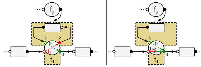
Figure 5.8.: Self-Activation with Data Node with Additional Incoming Channel
