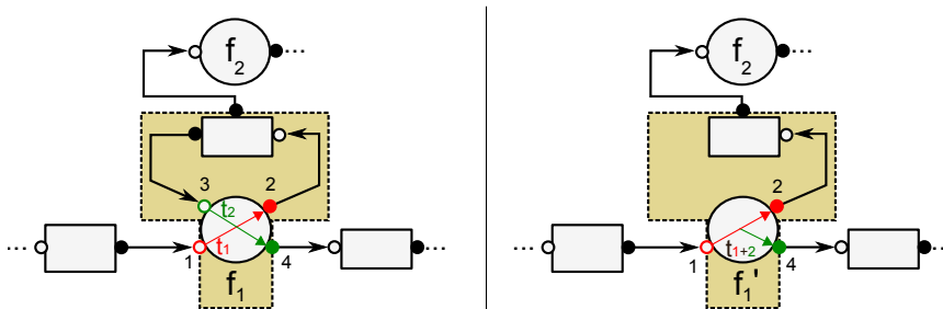
Figure 5.7.: Self-Activation with Data Node with Additional Outgoing Channel
