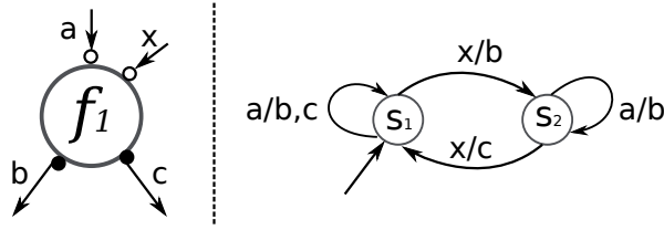
Figure 3.16.: Example for Causal Dependencies in Function Nodes
