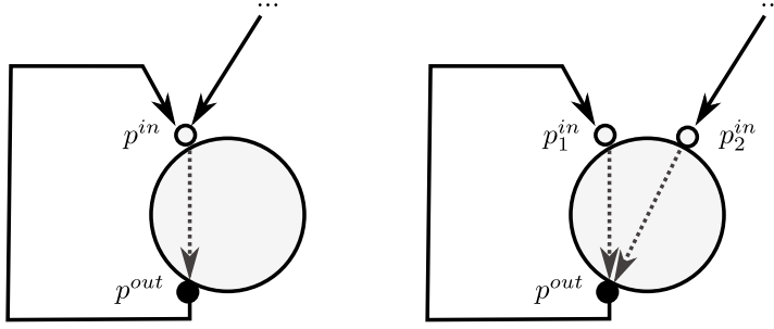
Figure 3.33.: Examples for Cyclic Causal Dependencies
