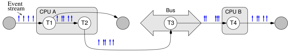
Figure 2.2.: Example for a Task Network (Source: [24])
