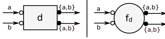
Figure 3.11.: Translation of Signal Data Node
