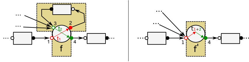
Figure 5.10.: Extension of Self-Activation Elimination to Multiple Input Channels
