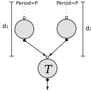
Figure 3.5.: Motivation for Offset in Event Models
