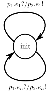
Figure 3.22.: Basic Channel Automaton TA(c)
