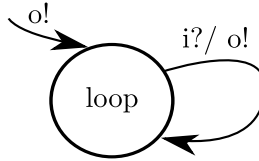
Figure 3.26.: Loop Automaton
