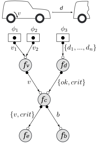
Figure 3.2.: Simple Example of an Adaptive Cruise Control (ACC) System
