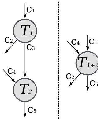
Figure 3.4.: Merging Example for a Complex Task Chain
