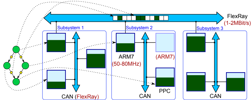
Figure 1.1.: Distributed Hardware Architecture
