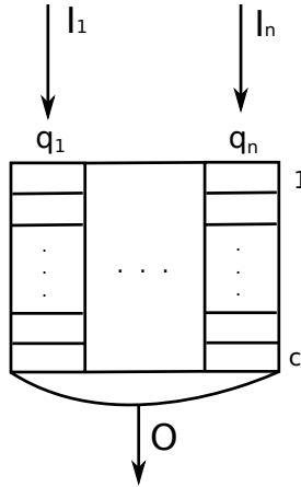
Figure 3.24.: Synchronization Buffer
