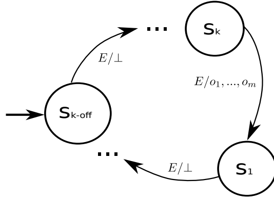
Figure 4.3.: Period Multiplier Transition System
