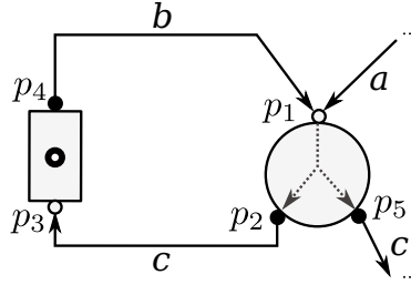
Figure 3.13.: Example of a Synchronization (AND) Loop
