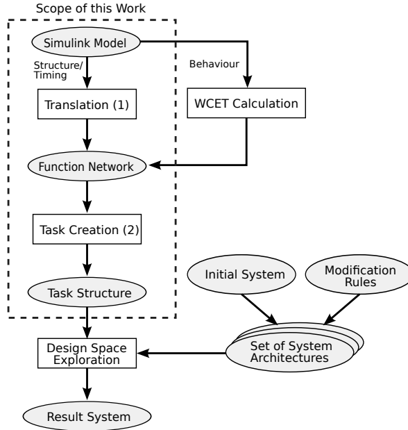
Figure 1.2.: Overview of Design Space Exploration Framework
