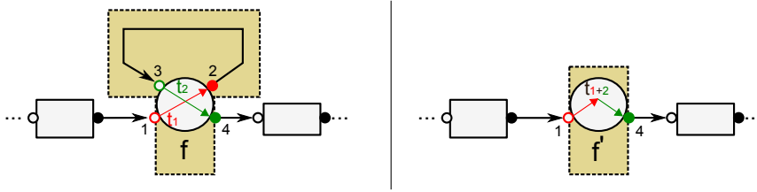
Figure 5.5.: Simple Self-Activation with Direct Channel
