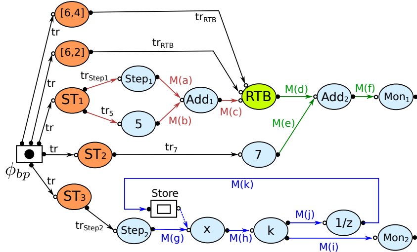
(b) Function Network Events representing Signal Updates
