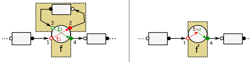
Figure 5.6.: Simple Self-Activation with Local Data Node
