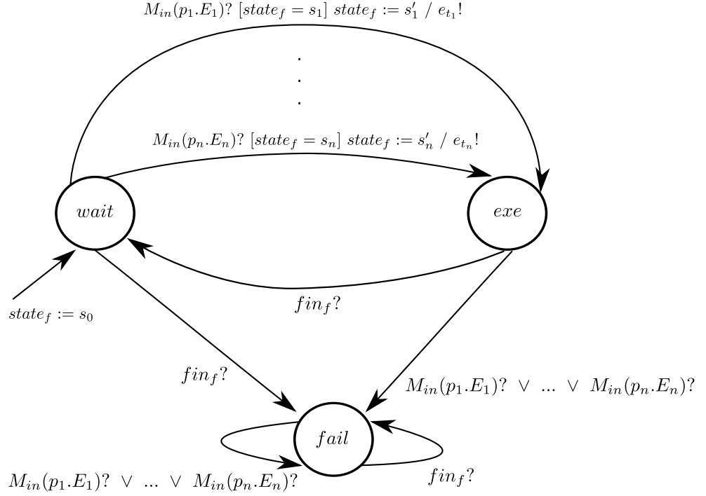
Figure 3.28.: Activation Automaton TA_{Activate}
