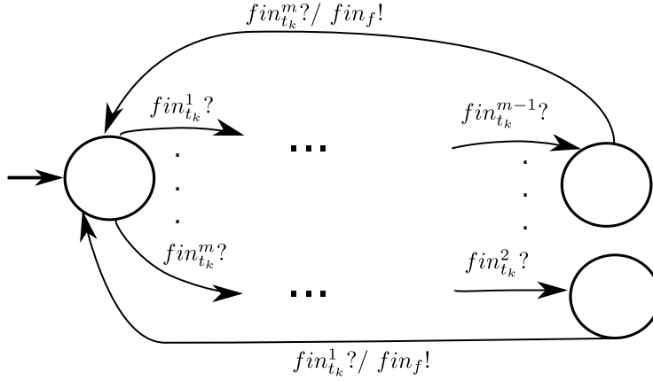
Figure 3.30.: Finish Automaton TA_{Finish}^{t_k} for Transition t_k
