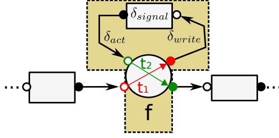
Figure 5.9.: Delays for Self-Activation
