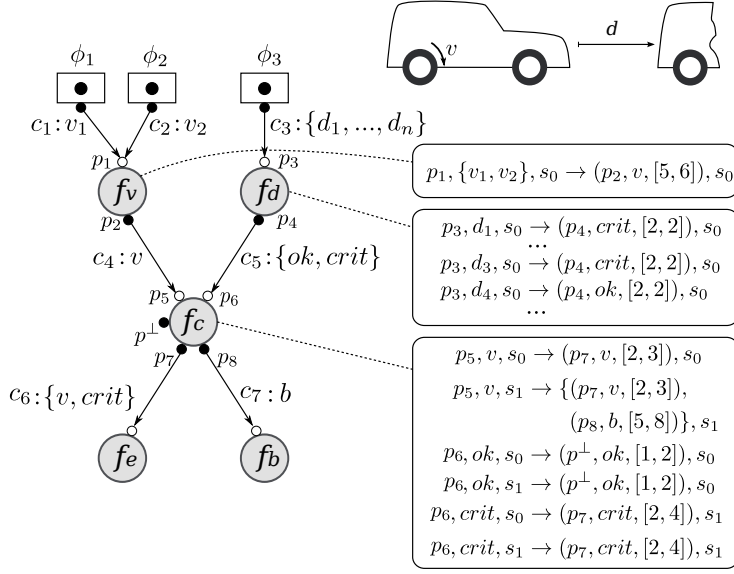
Figure 3.7.: Simple Function Network Model of an Adaptive Cruise Control System
