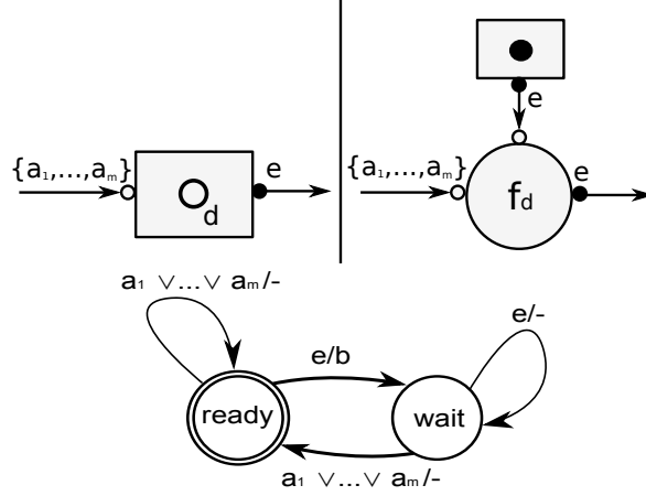
Figure 3.12.: Translation of Finite Source Data Node
