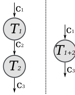
Figure 3.3.: Merging Example for a Simple Task Chain
