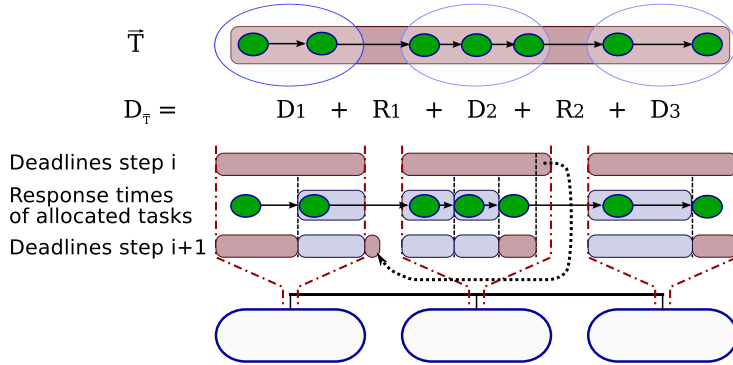
Figure 6.4.: Deadline Synthesis and Re-Synthesis (Source:[11])
