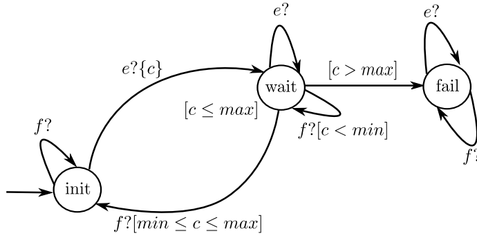
Figure 3.17.: Observer Automaton for RSL 'F1' Pattern [65]
