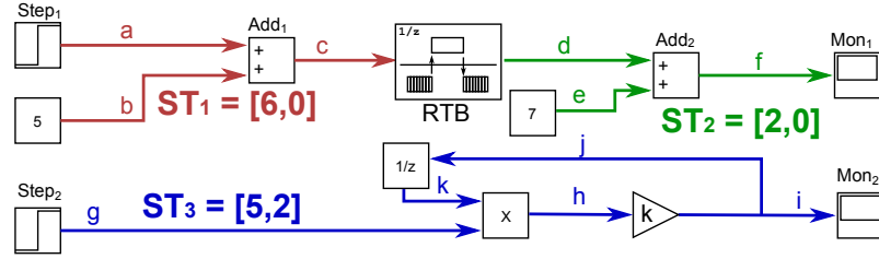
(a) Signals in a Simulink Block Diagram
