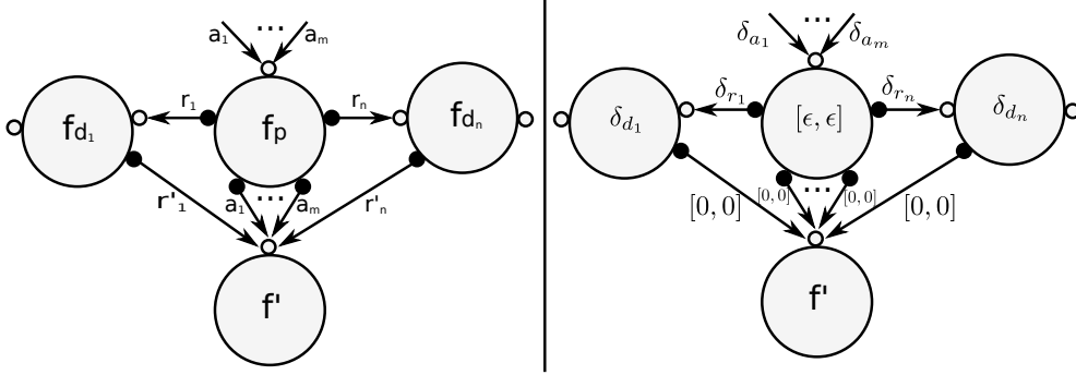
Figure 5.4.: Left: Translation of Read Channels into Basic Function Network Right: Delays of Reading Data Nodes
