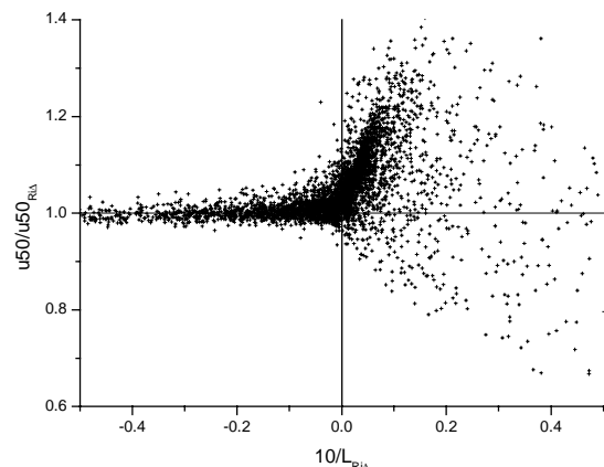
Figure 3: Ratio of measured and calculated wind speed at 50m height versus atmospheric stability; the wind speed has been calculated from the 10m wind speed using the Charnock roughness description and the stability determined via Ri number
