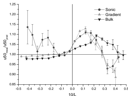
Figure 4: Comparison of different methods to determine the atmospheric stability; ratios of measured and calculated wind speeds at 50m height versus atmospheric stability are shown
