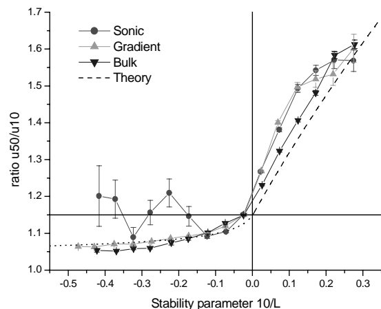
Figure 2: Bin-averaged measured wind speed u_{50}/u_{10} versus stability parameter 10/L determined with three different methods
